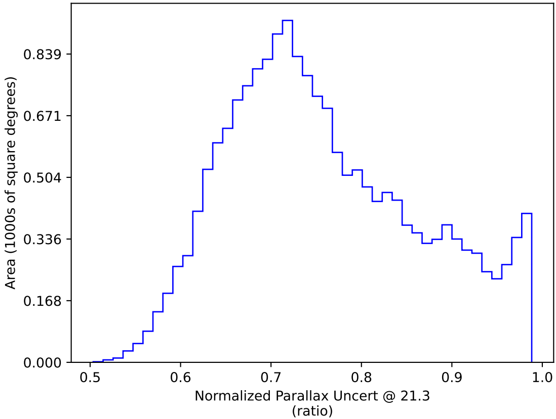
ddf_acor_sf25_lsf30_lsr10_v3.4_10yrs WFD y band only: Normalized Parallax Uncert @ 21.3
