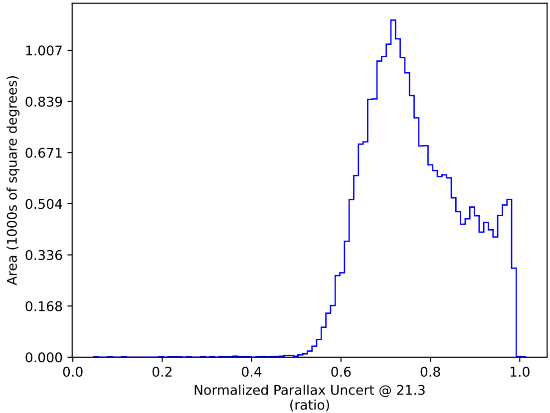
ddf_acor_sf25_lsf30_lsr10_v3.4_10yrs All sky y band only: Normalized Parallax Uncert @ 21.3
