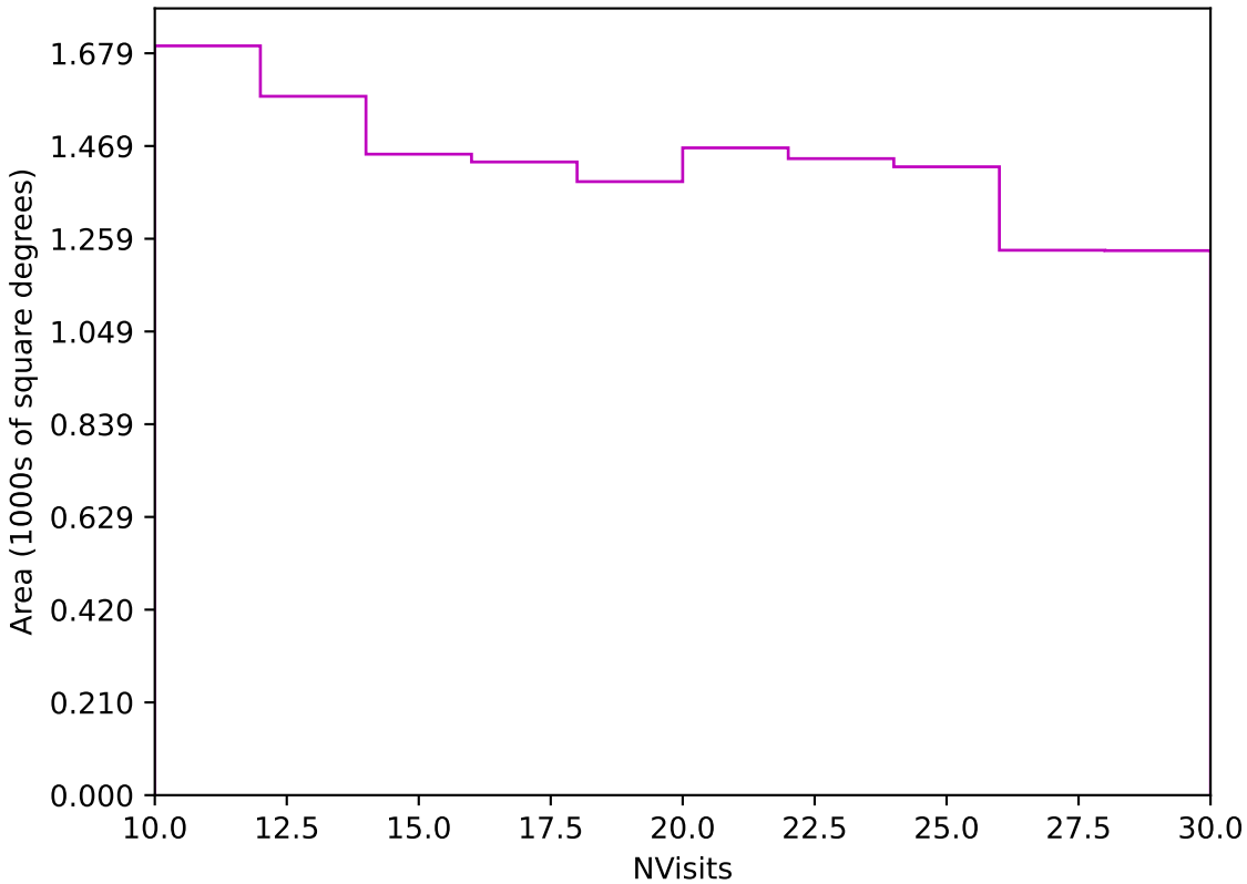
ddf_acor_sf25_lsf30_lsr10_v3.4_10yrs Yr 3-4 z band: NVisits
