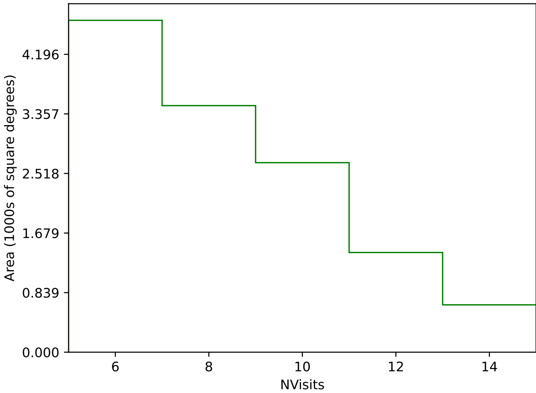
ddf_acor_sf25_lsf30_lsr10_v3.4_10yrs Yr 3-4 g band: NVisits
