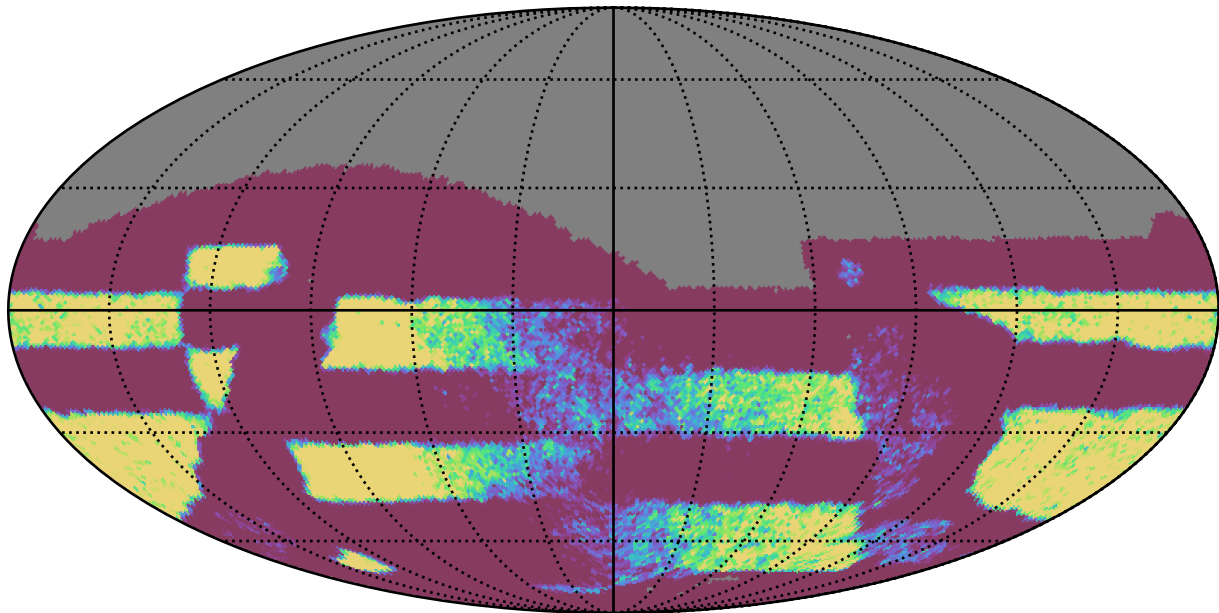
ddf_acor_sf25_lsf30_lsr10_v3.4_10yrs Yr 3-4 all bands: NVisits
