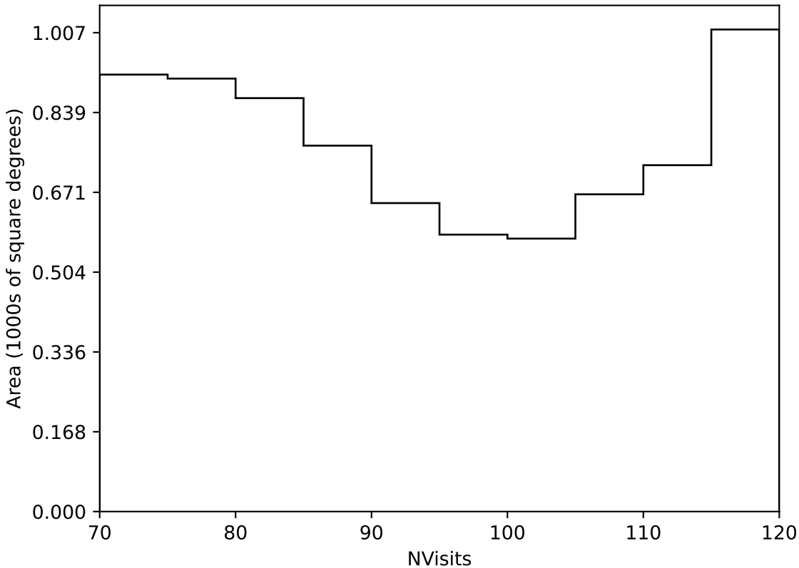
ddf_acor_sf25_lsf30_lsr10_v3.4_10yrs Yr 3-4 all bands: NVisits
