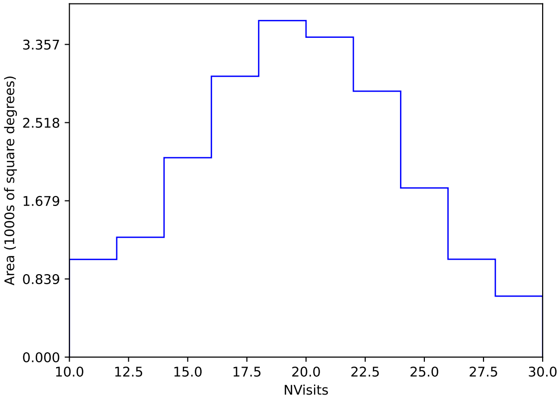
ddf_acor_sf25_lsf30_lsr10_v3.4_10yrs Yr 1 y band: NVisits
