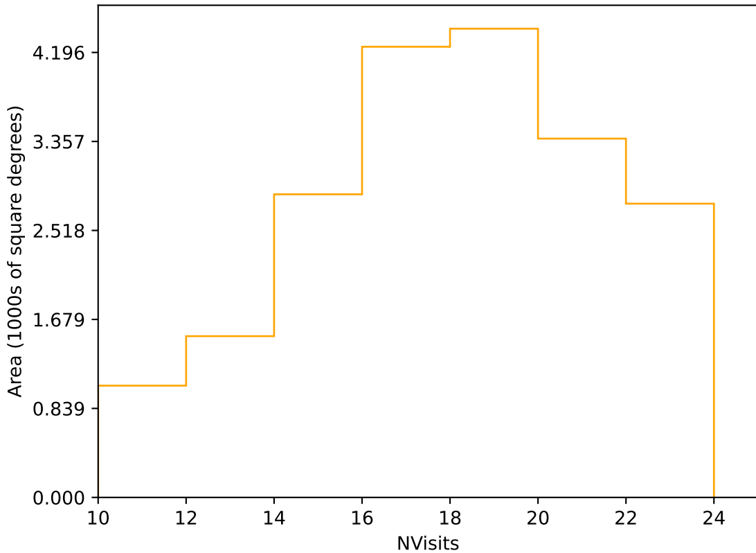
ddf_acor_sf25_lsf30_lsr10_v3.4_10yrs Yr 1 r band: NVisits
