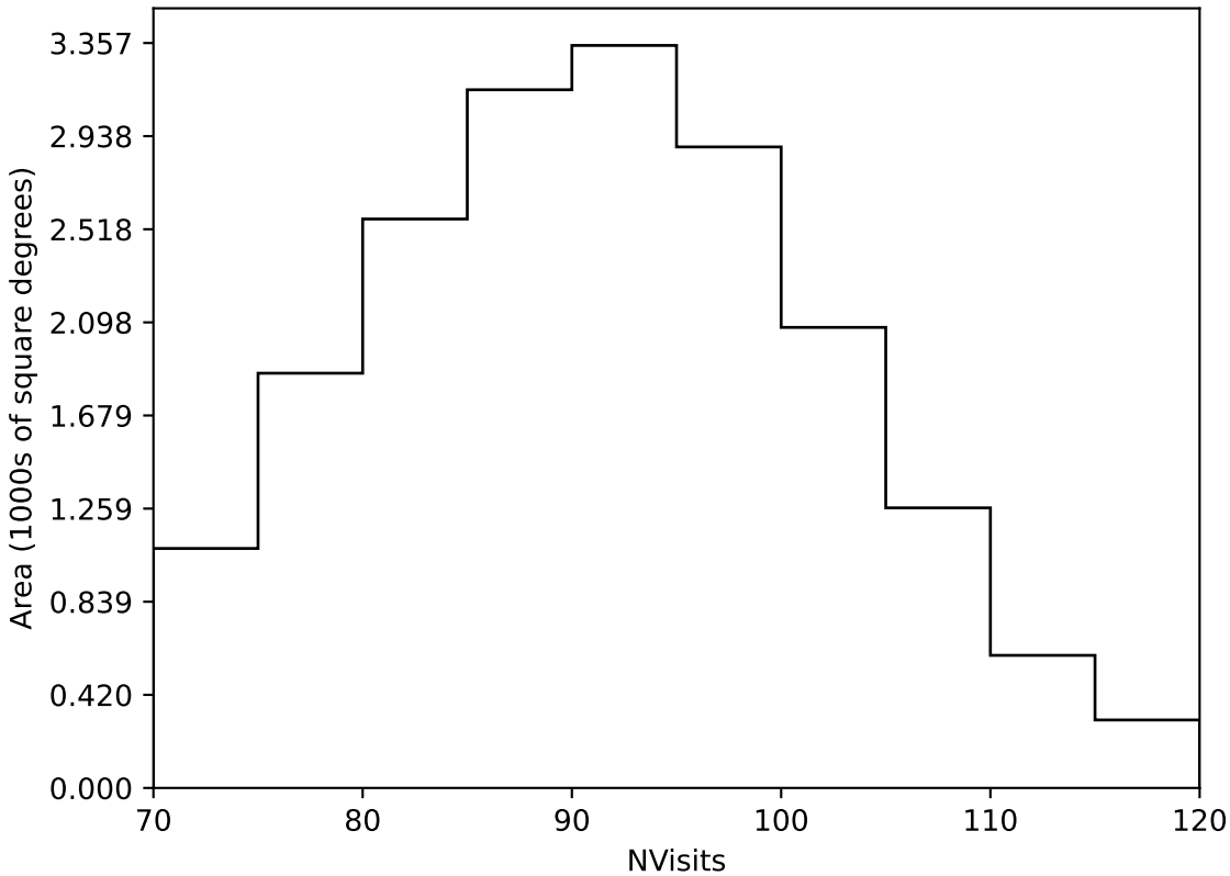
ddf_acor_sf25_lsf30_lsr10_v3.4_10yrs Yr 1 all bands: NVisits
