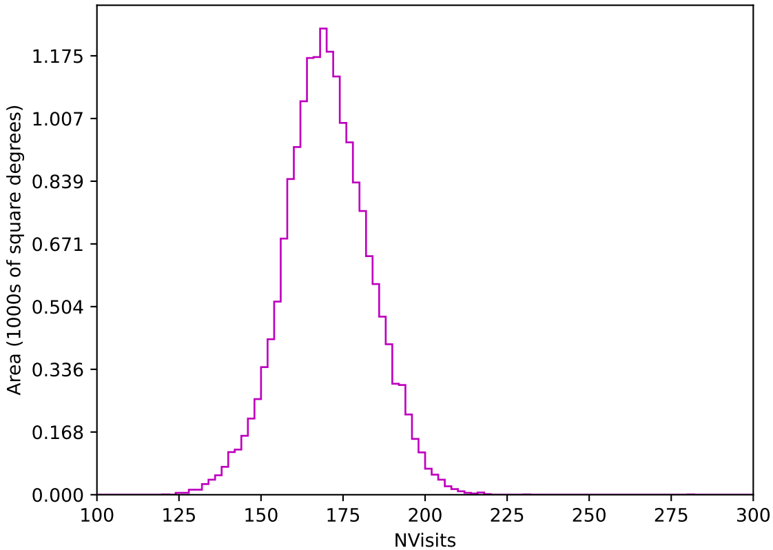
ddf_acor_sf25_lsf30_lsr10_v3.4_10yrs WFD z band: NVisits
