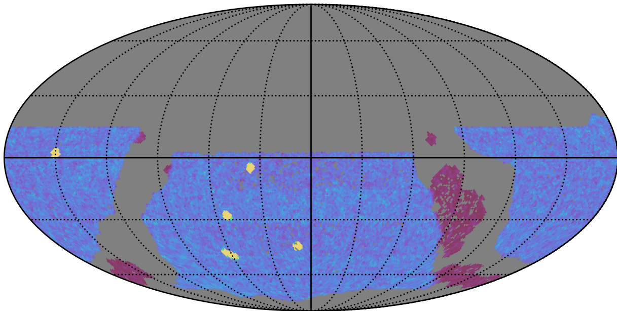
ddf_acor_sf25_lsf30_lsr10_v3.4_10yrs WFD y band: NVisits
