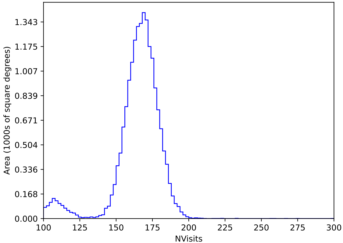
ddf_acor_sf25_lsf30_lsr10_v3.4_10yrs WFD y band: NVisits
