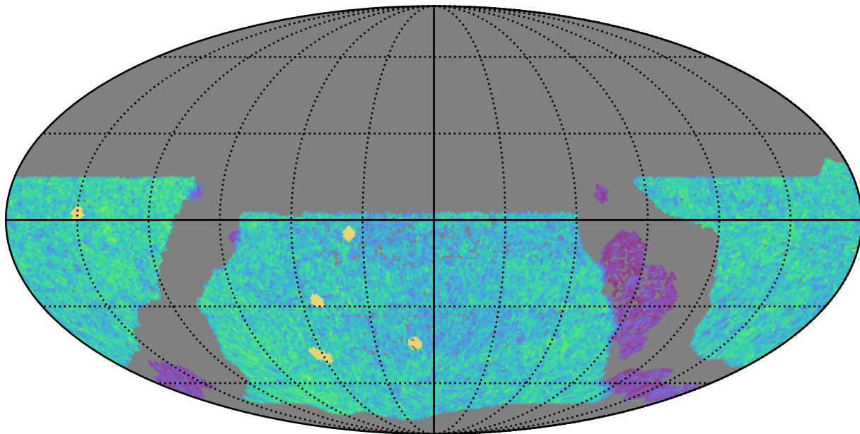
ddf_acor_sf25_lsf30_lsr10_v3.4_10yrs WFD u band: NVisits
