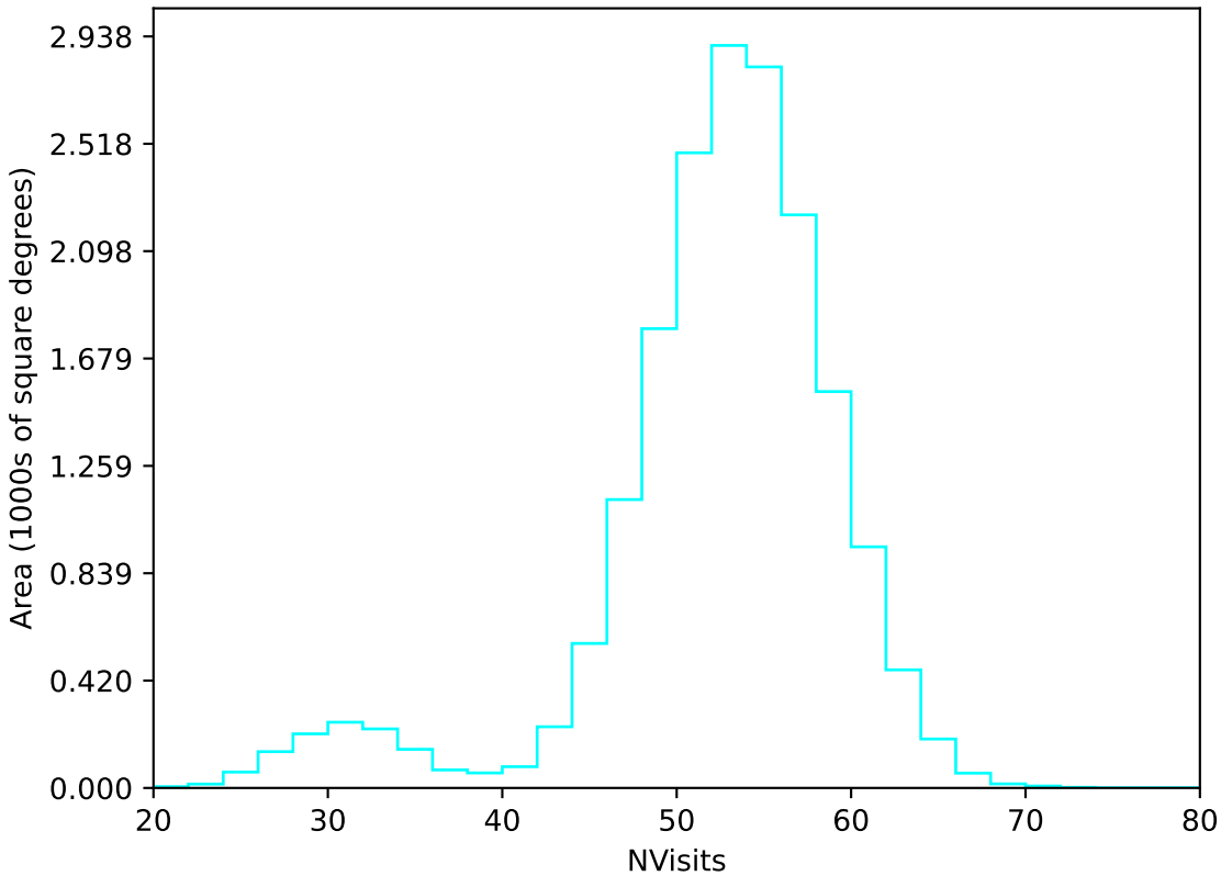
ddf_acor_sf25_lsf30_lsr10_v3.4_10yrs WFD u band: NVisits
