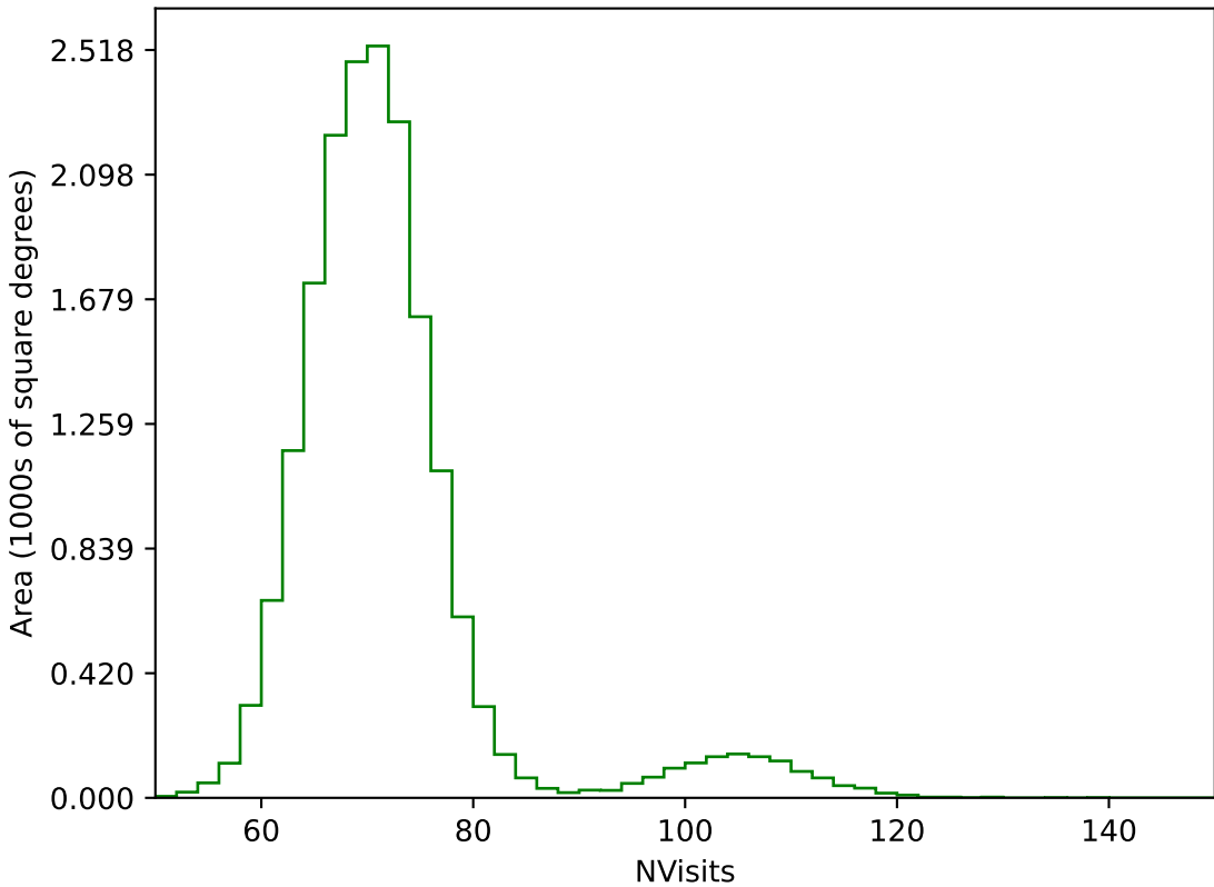
ddf_acor_sf25_lsf30_lsr10_v3.4_10yrs WFD g band: NVisits
