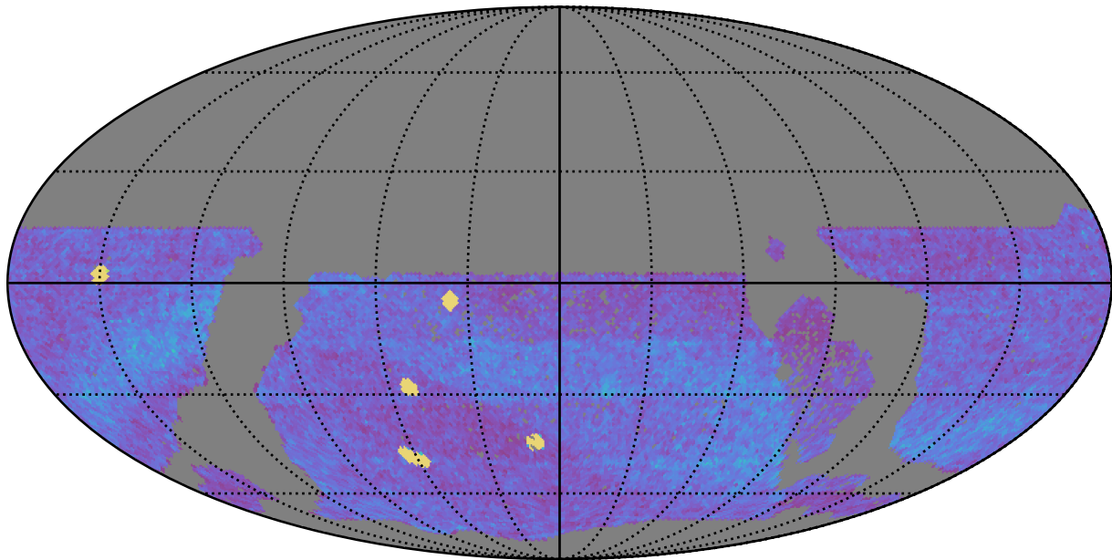
ddf_acor_sf25_lsf30_lsr10_v3.4_10yrs WFD all bands: NVisits
