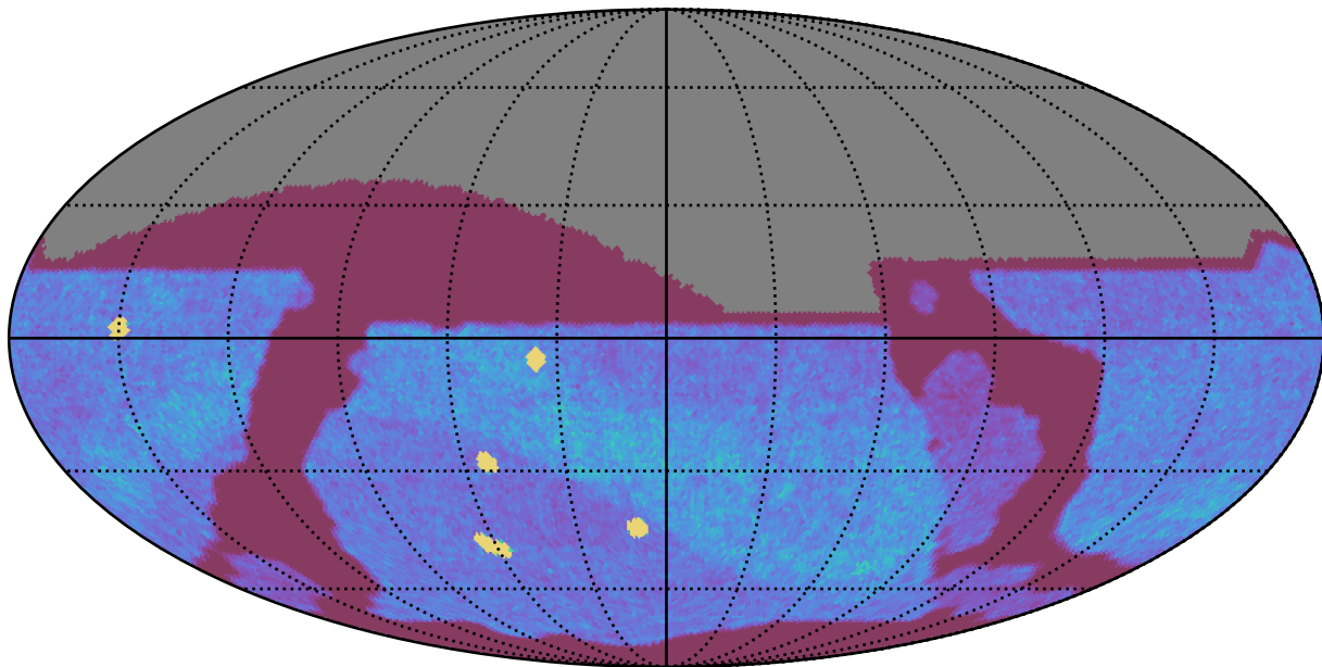
ddf_acor_sf25_lsf30_lsr10_v3.4_10yrs All sky z band: NVisits
