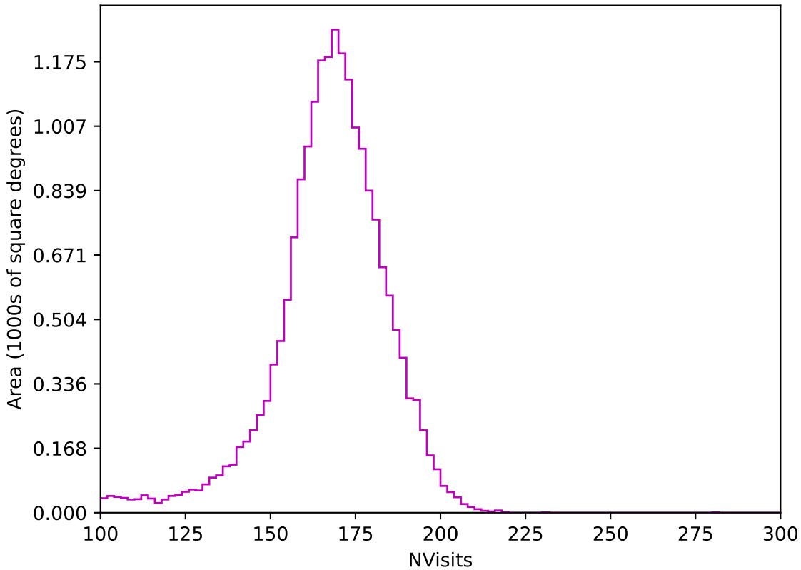
ddf_acor_sf25_lsf30_lsr10_v3.4_10yrs All sky z band: NVisits
