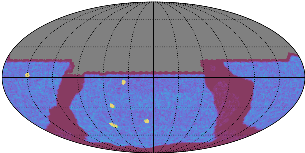
ddf_acor_sf25_lsf30_lsr10_v3.4_10yrs All sky y band: NVisits
