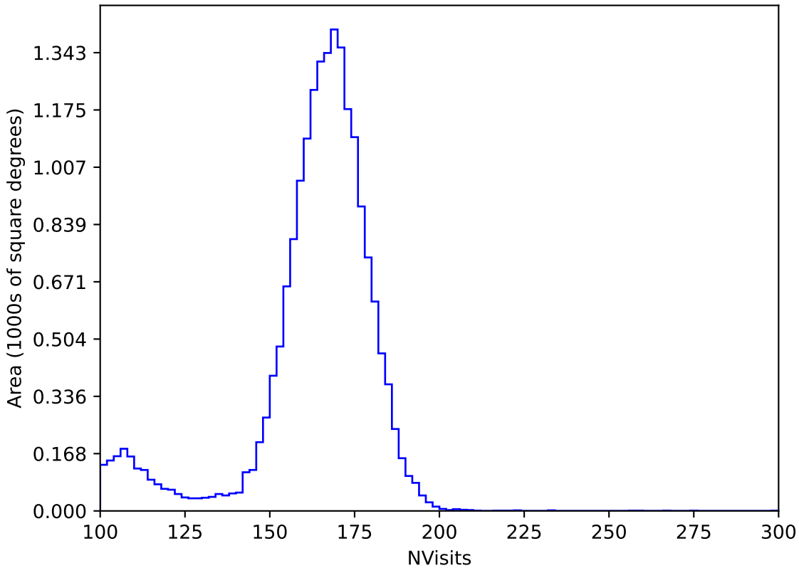
ddf_acor_sf25_lsf30_lsr10_v3.4_10yrs All sky y band: NVisits
