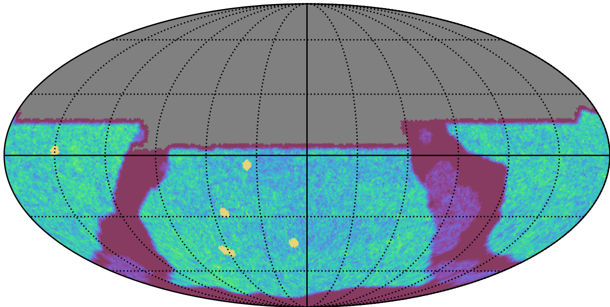
ddf_acor_sf25_lsf30_lsr10_v3.4_10yrs All sky u band: NVisits
