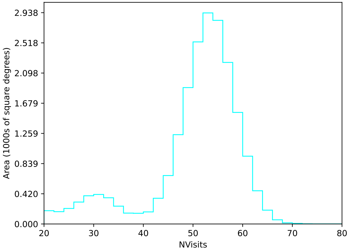
ddf_acor_sf25_lsf30_lsr10_v3.4_10yrs All sky u band: NVisits
