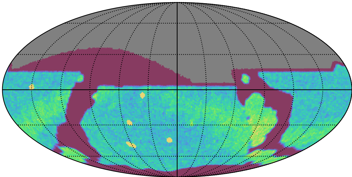
ddf_acor_sf25_lsf30_lsr10_v3.4_10yrs All sky r band: NVisits
