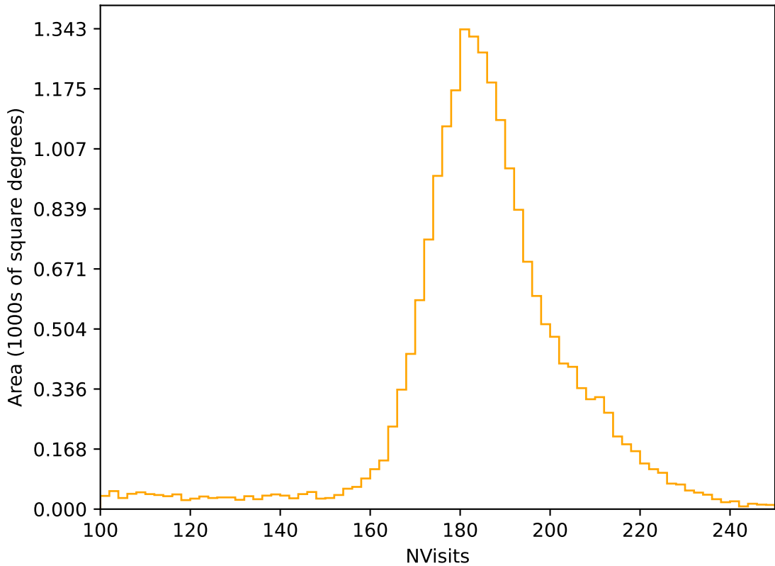
ddf_acor_sf25_lsf30_lsr10_v3.4_10yrs All sky r band: NVisits
