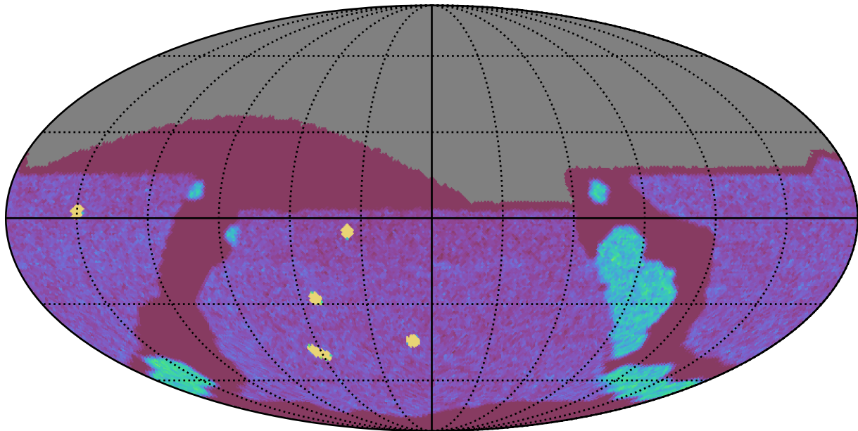
ddf_acor_sf25_lsf30_lsr10_v3.4_10yrs All sky g band: NVisits
