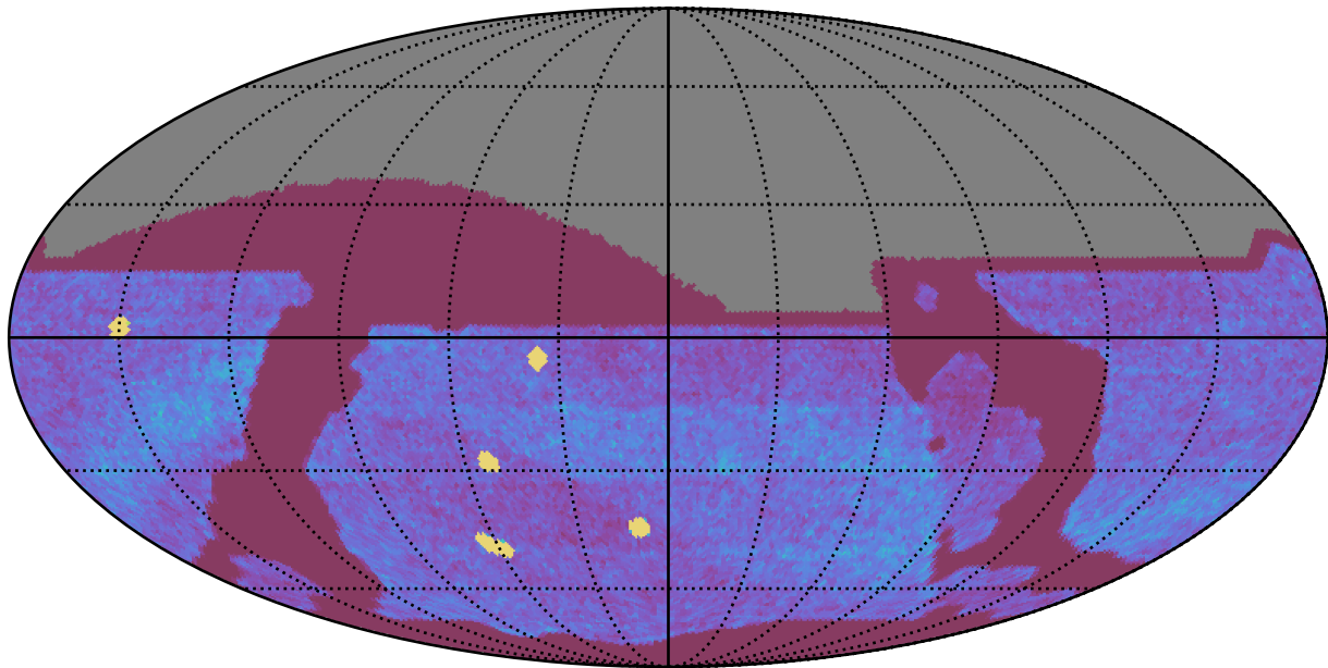
ddf_acor_sf25_lsf30_lsr10_v3.4_10yrs All sky all bands: NVisits
