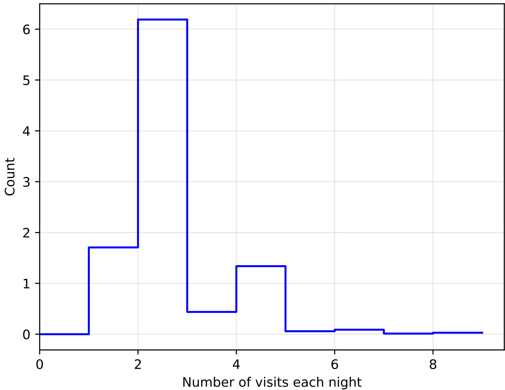
ddf_acor_sf25_lsf30_lsr10_v3.4_10yrs All sky: NVisitsPerNight 1e6
