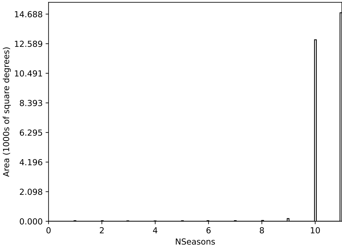
ddf_acor_sf25_lsf30_lsr10_v3.4_10yrs All sky all bands: NSeasons
