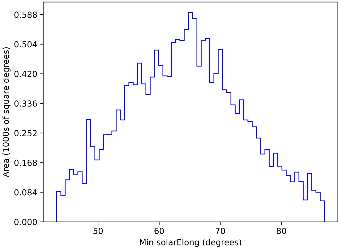
ddf_acor_sf25_lsf30_lsr10_v3.4_10yrs WFD y band: Min solarElong
