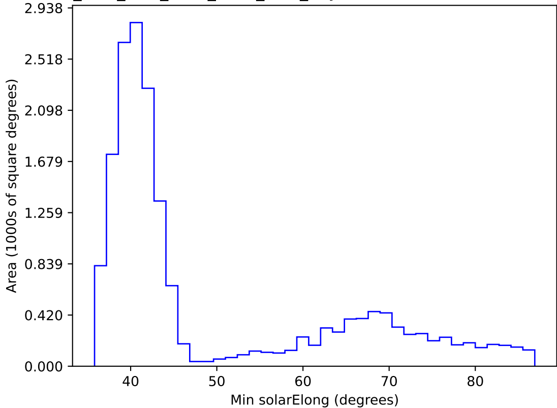
ddf_acor_sf25_lsf30_lsr10_v3.4_10yrs WFD i band: Min solarElong
