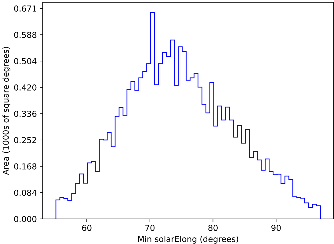
ddf_acor_sf25_lsf30_lsr10_v3.4_10yrs WFD g band: Min solarElong
