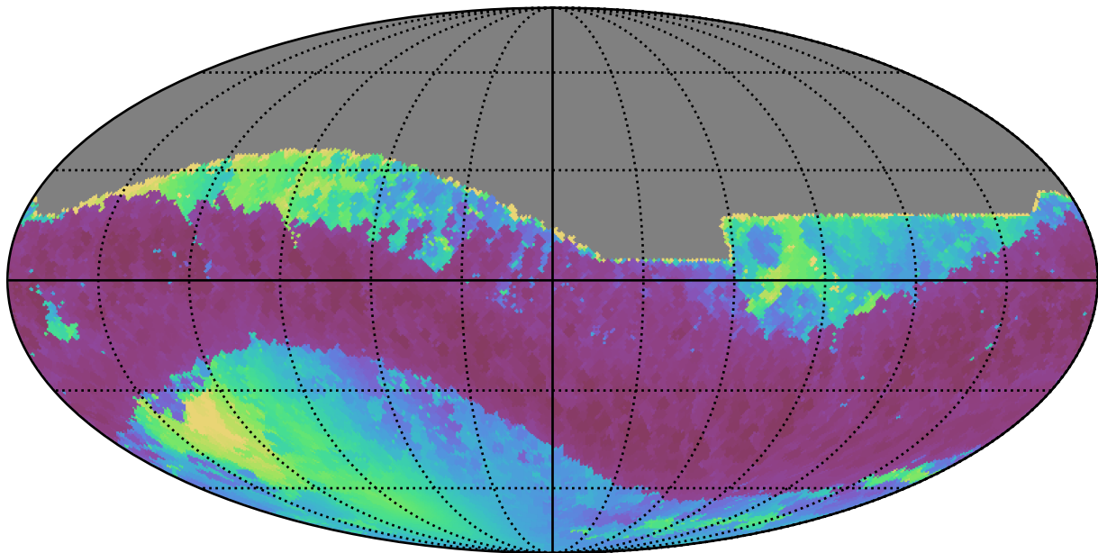
ddf_acor_sf25_lsf30_lsr10_v3.4_10yrs All sky z band: Min solarElong
