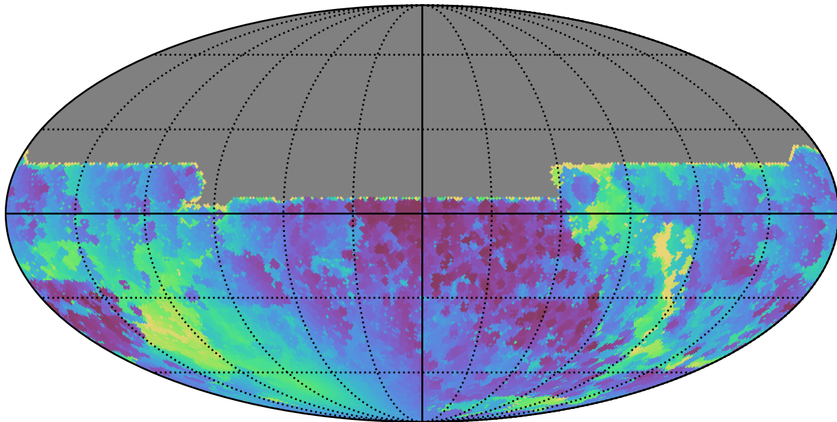
ddf_acor_sf25_lsf30_lsr10_v3.4_10yrs All sky y band: Min solarElong
