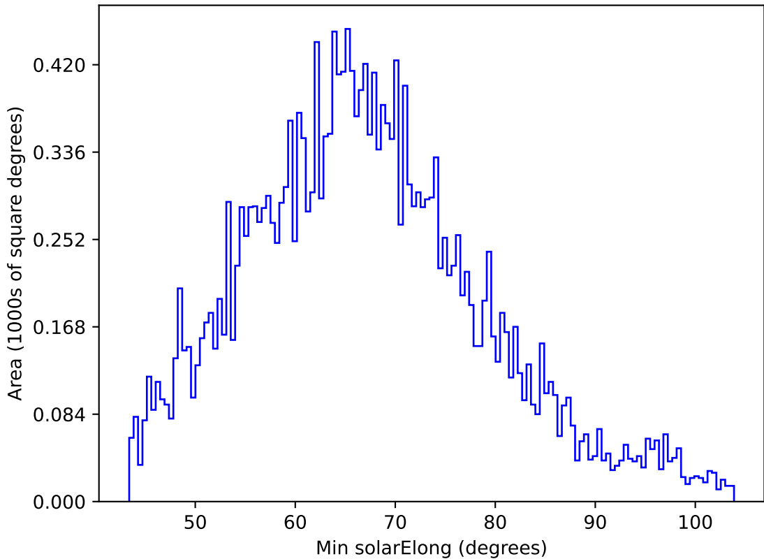
ddf_acor_sf25_lsf30_lsr10_v3.4_10yrs All sky y band: Min solarElong
