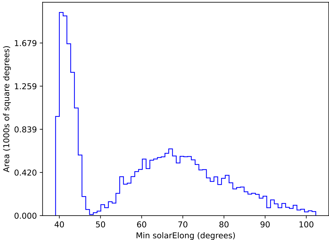
ddf_acor_sf25_lsf30_lsr10_v3.4_10yrs All sky r band: Min solarElong
