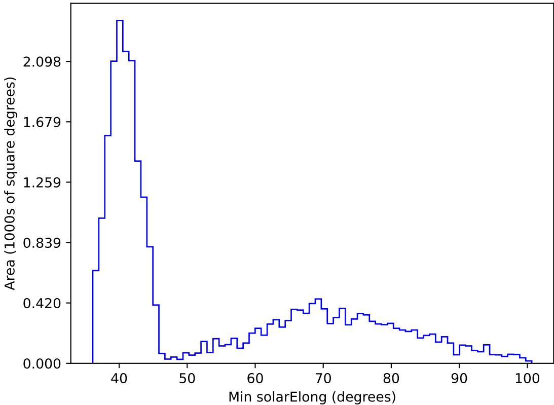
ddf_acor_sf25_lsf30_lsr10_v3.4_10yrs All sky i band: Min solarElong
