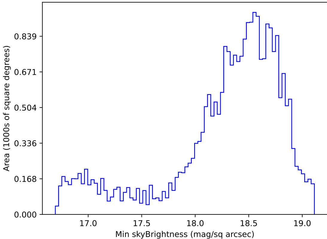
ddf_acor_sf25_lsf30_lsr10_v3.4_10yrs Yr 1 z band: Min skyBrightness
