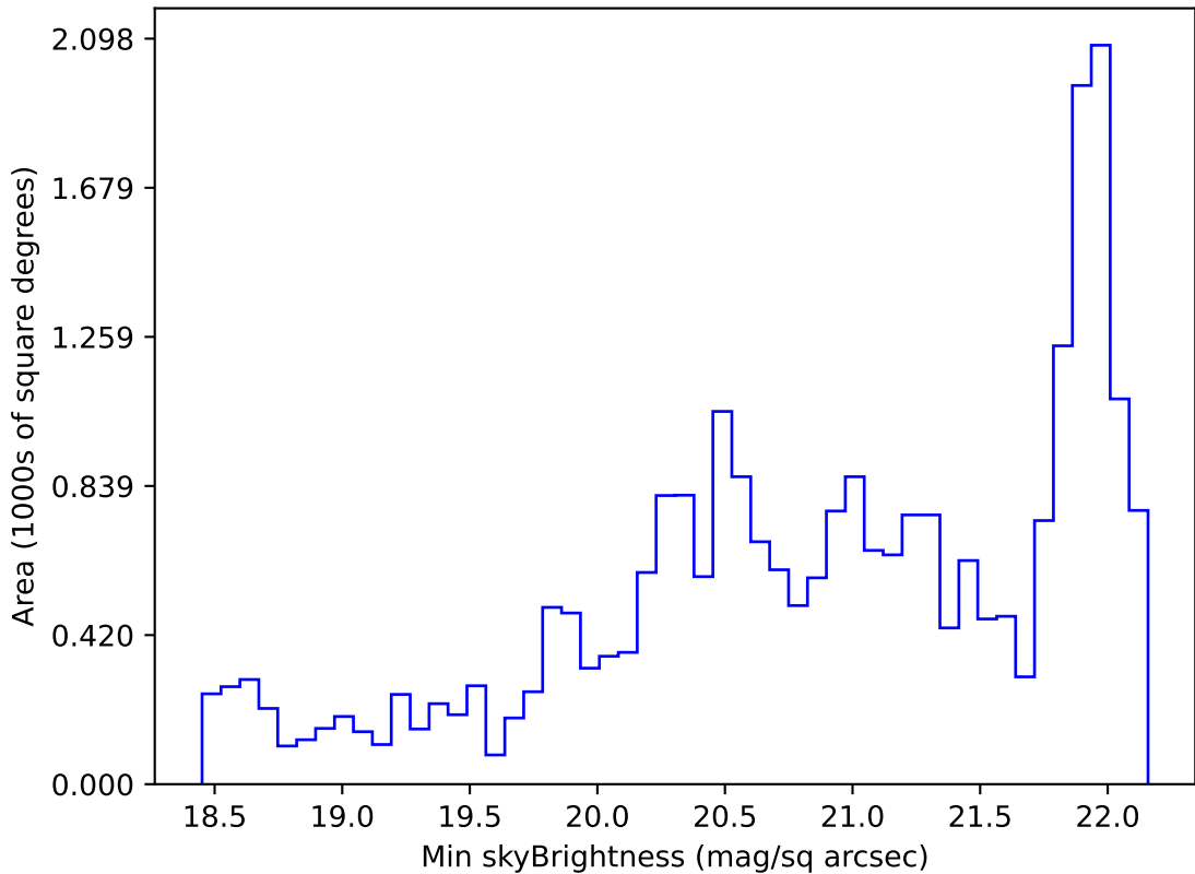
ddf_acor_sf25_lsf30_lsr10_v3.4_10yrs Yr 1 g band: Min skyBrightness
