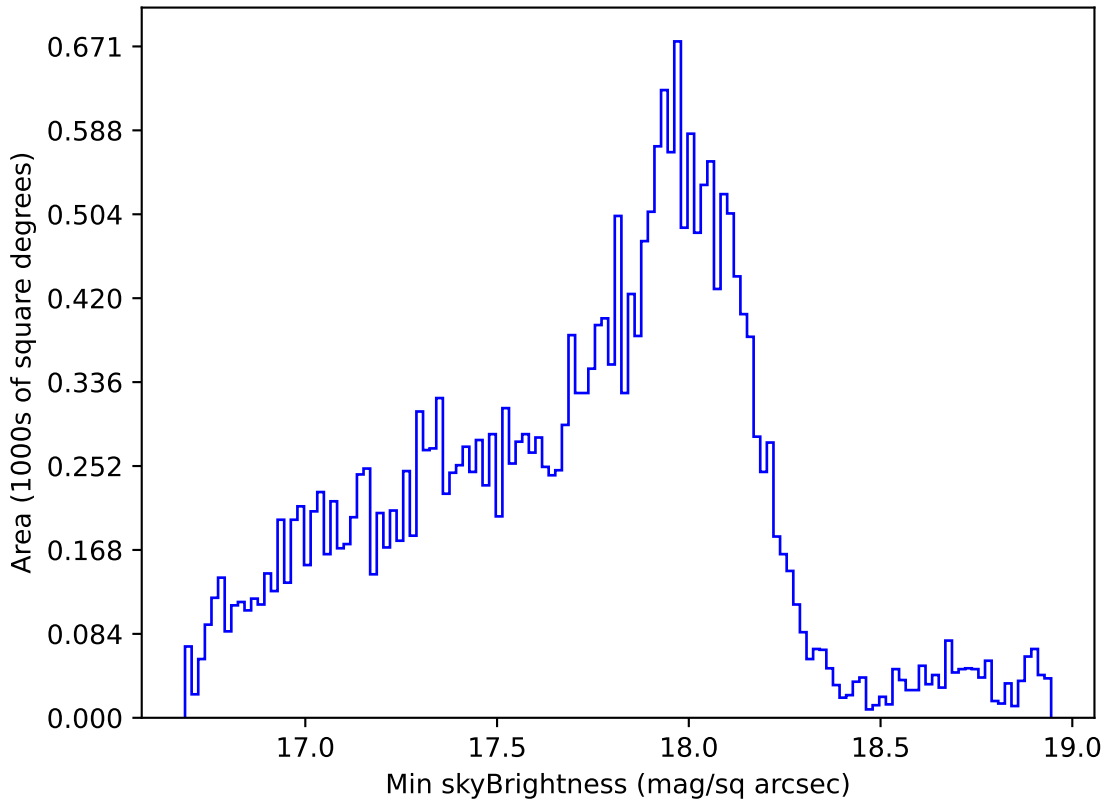
ddf_acor_sf25_lsf30_lsr10_v3.4_10yrs Yr 1 all bands: Min skyBrightness
