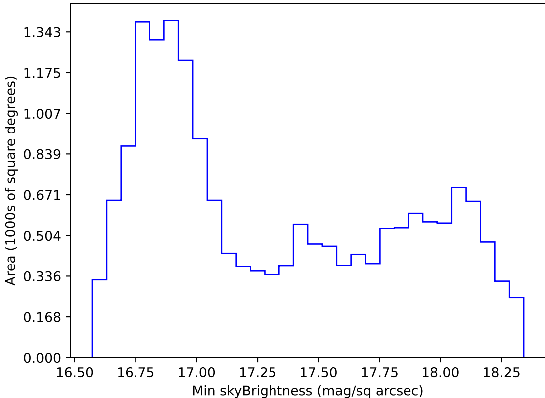
ddf_acor_sf25_lsf30_lsr10_v3.4_10yrs WFD z band: Min skyBrightness
