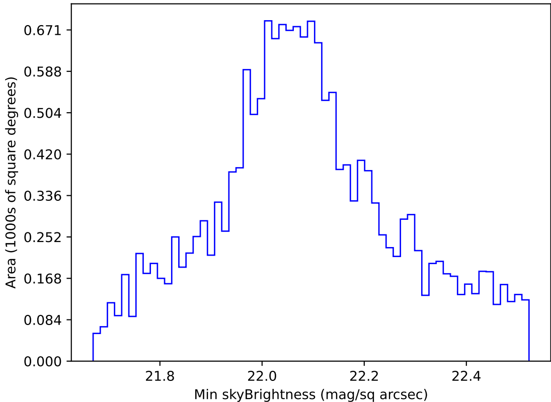
ddf_acor_sf25_lsf30_lsr10_v3.4_10yrs WFD u band: Min skyBrightness
