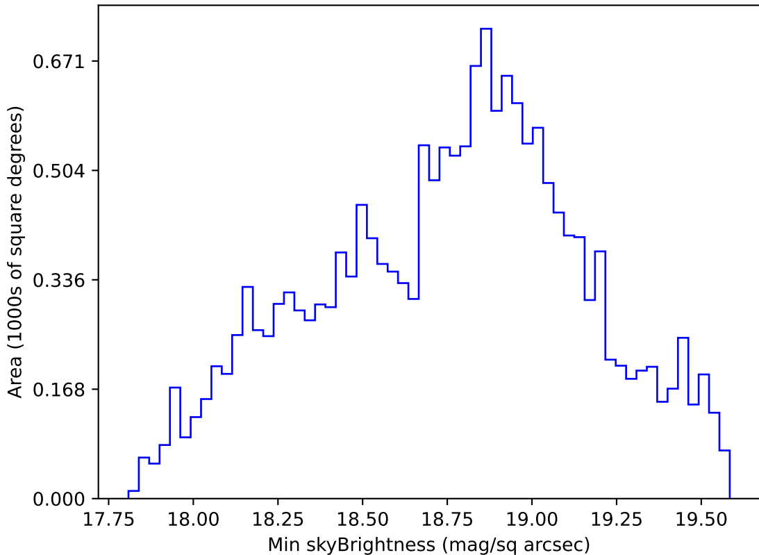
ddf_acor_sf25_lsf30_lsr10_v3.4_10yrs WFD r band: Min skyBrightness
