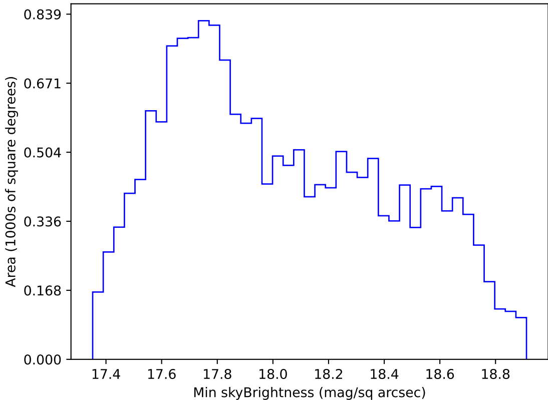
ddf_acor_sf25_lsf30_lsr10_v3.4_10yrs WFD i band: Min skyBrightness
