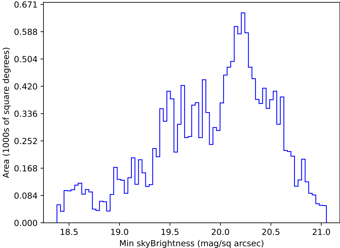
ddf_acor_sf25_lsf30_lsr10_v3.4_10yrs WFD g band: Min skyBrightness
