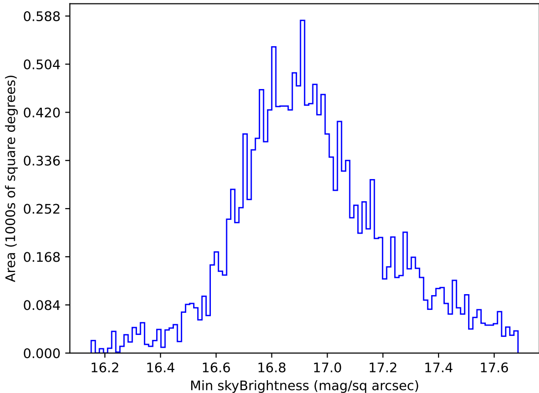
ddf_acor_sf25_lsf30_lsr10_v3.4_10yrs WFD all bands: Min skyBrightness
