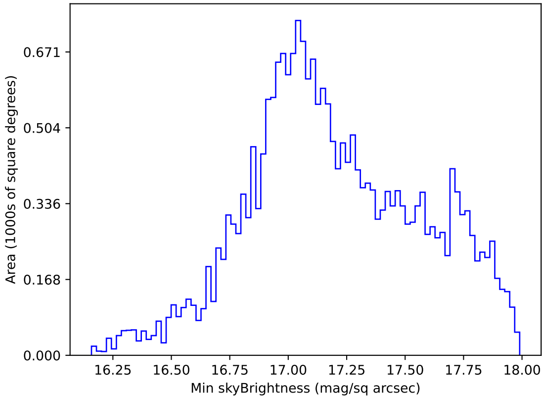
ddf_acor_sf25_lsf30_lsr10_v3.4_10yrs All sky y band: Min skyBrightness
