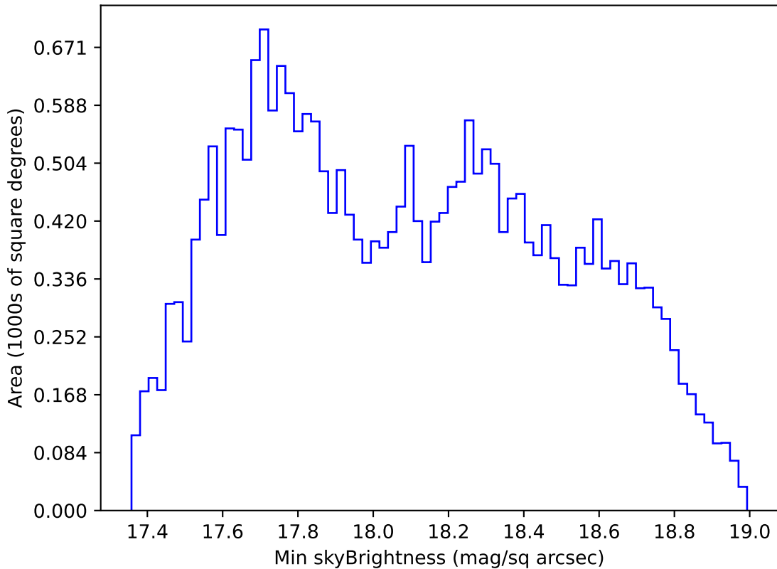
ddf_acor_sf25_lsf30_lsr10_v3.4_10yrs All sky i band: Min skyBrightness
