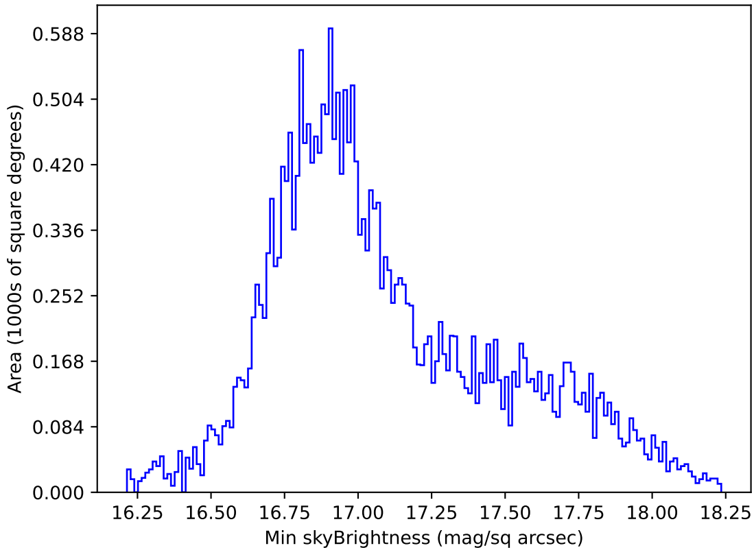
ddf_acor_sf25_lsf30_lsr10_v3.4_10yrs All sky all bands: Min skyBrightness
