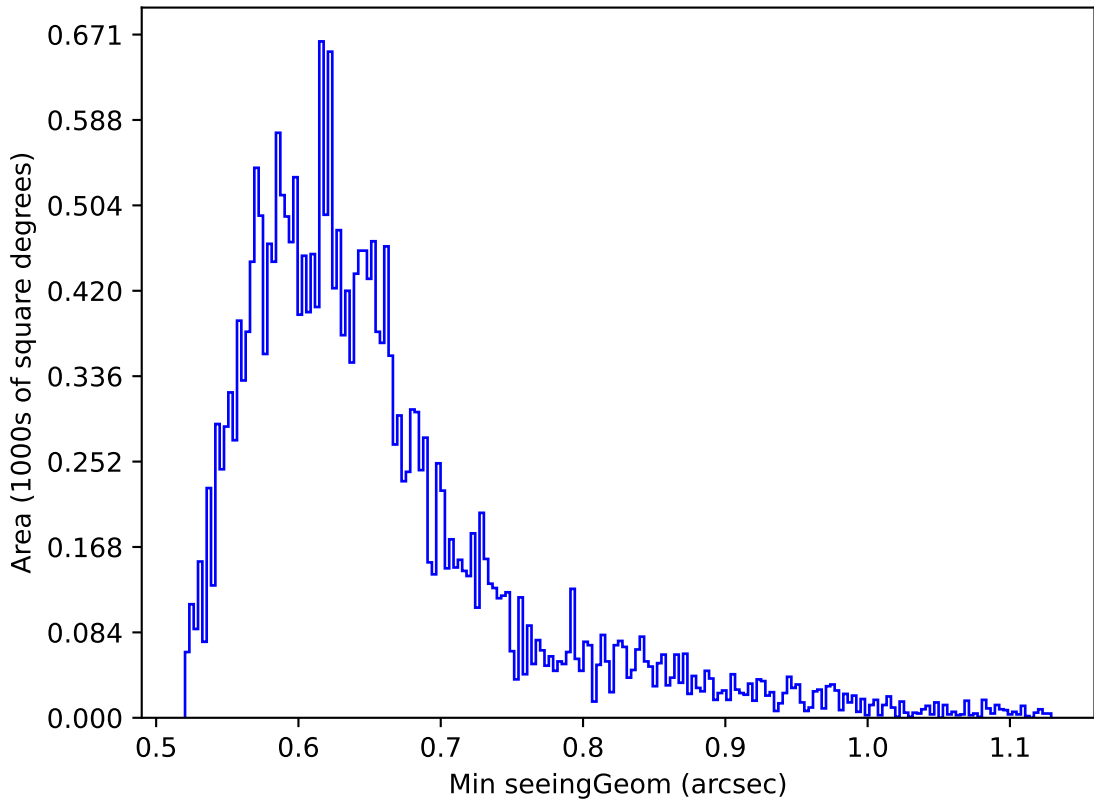
ddf_acor_sf25_ls30_lsr10_v3.4_10yrs Yr 1 z band: Min seeingGeom
