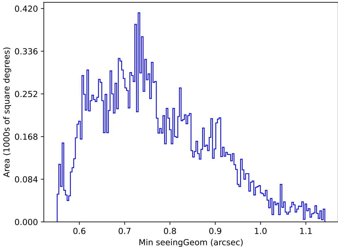
ddf_acor_sf25_lsf30_lsr10_v3.4_10yrs Yr 1 u band: Min seeingGeom
